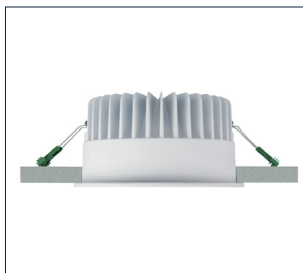
Installation detail
